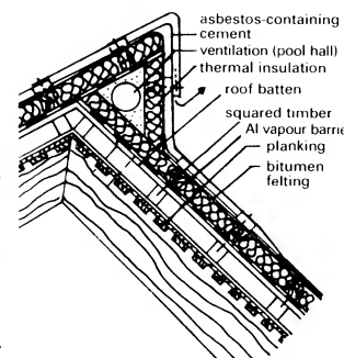
11 Ridge ventilation on a sloping cold roof (indoor swimming pool)
